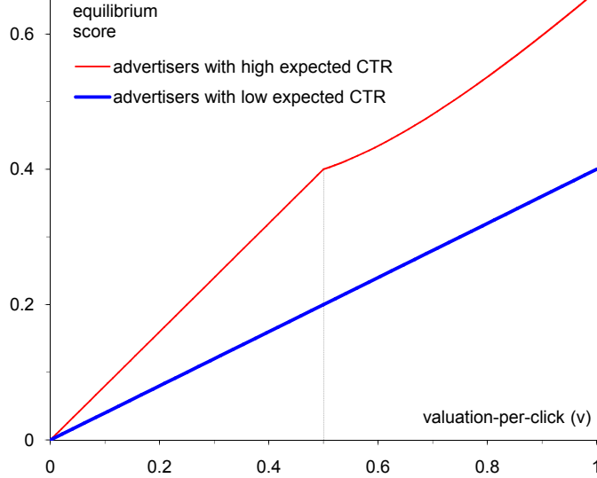
Figure 1: Equilibrium Bidding Functions
