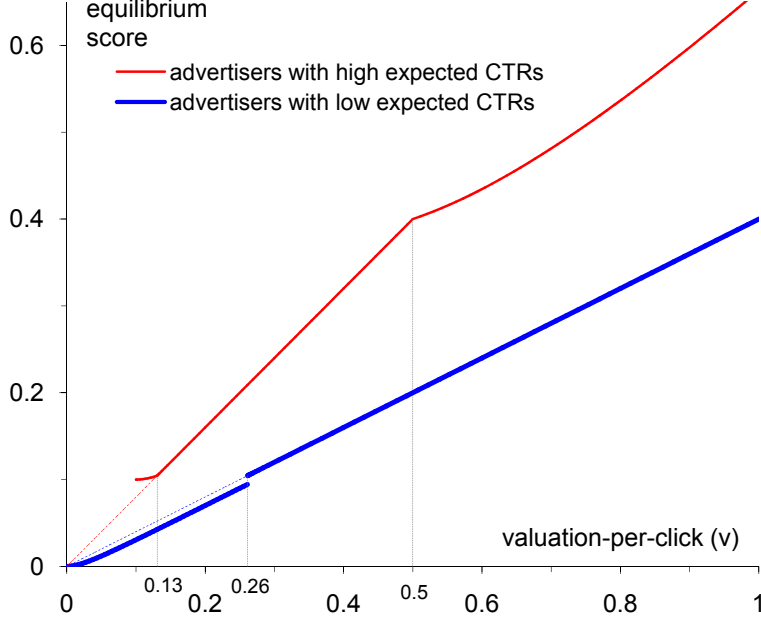
Figure 2: Equilibrium Bidding Functions with Minimum Bids
